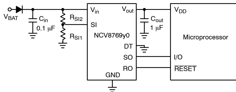
Figure 1. Application Circuit
