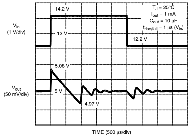
Figure 14. Line Transients
