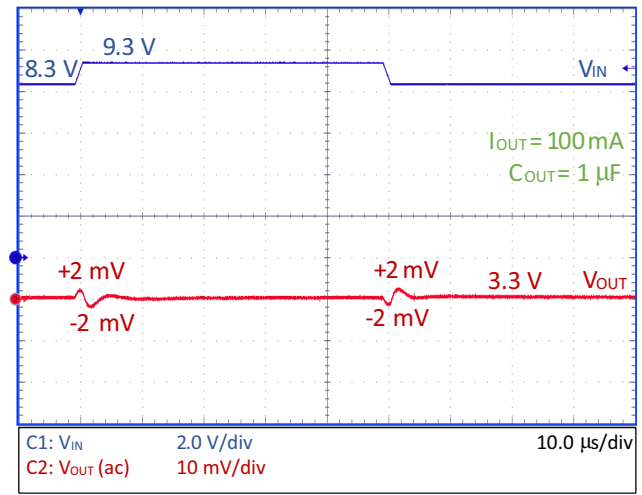
Figure 35. Line Transient – NCP730–3.3 V
