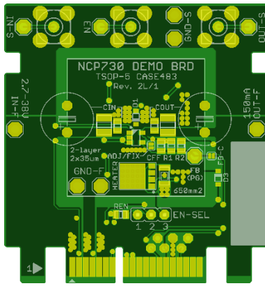
Figure 91. NCV8730 Demo Board (2 layer, rev. 1) – PCB Top Layer
