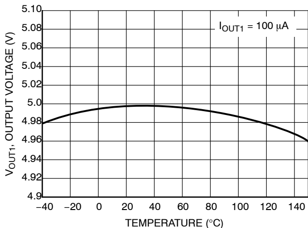
Figure 12. Output Voltage LDO1 vs Temperature
