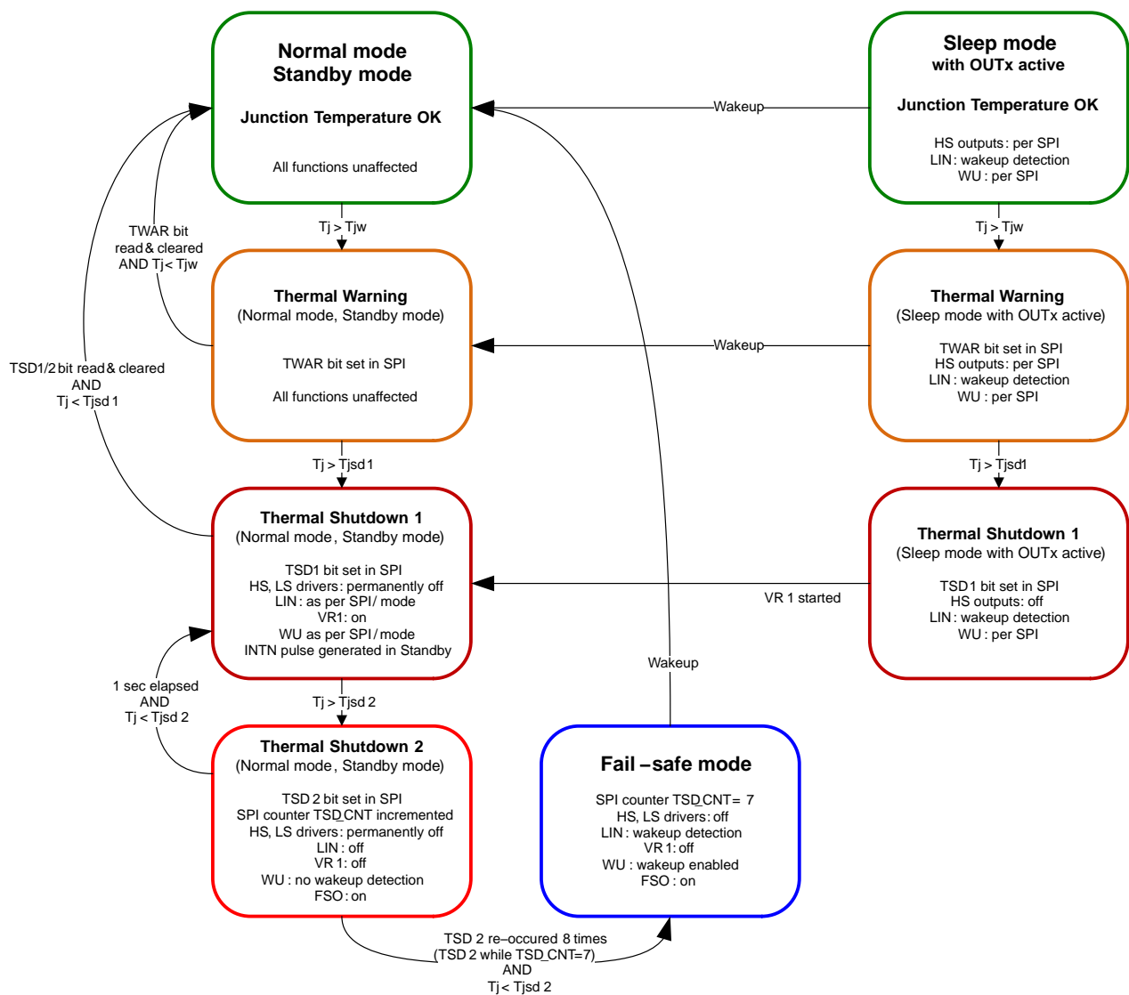
Figure 19. Thermal Protection
