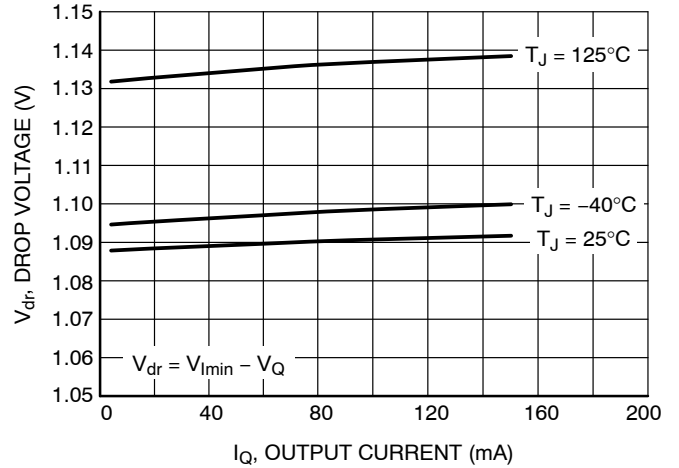
Figure 34. Drop Voltage vs. Output Current
