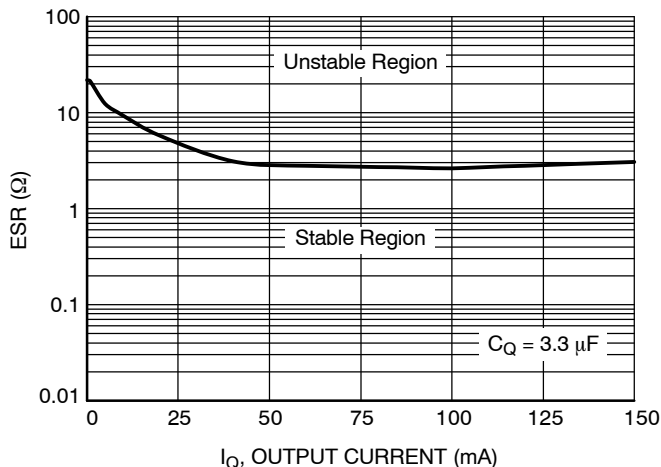
Figure 12. Output Stability with Output Capacitor ESR
