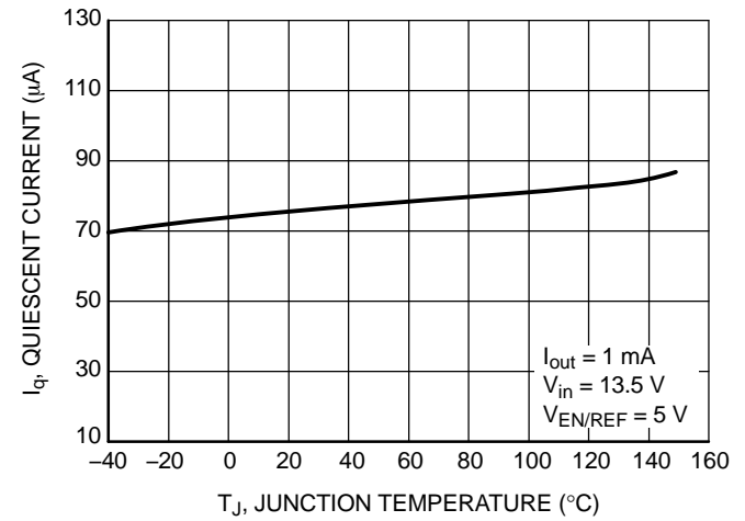
Figure 18. Current Consumption I_q vs. Junction Temperature T_J
