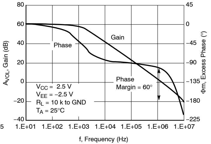
Figure 5. Gain and Phase vs. Frequency
