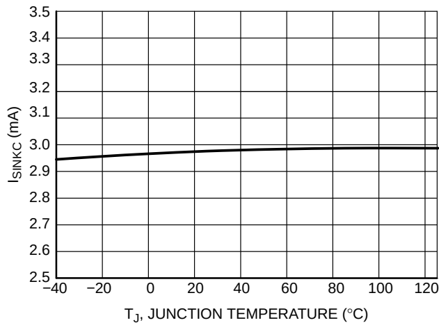
Figure 23. Current OTA Current Sink Capability
