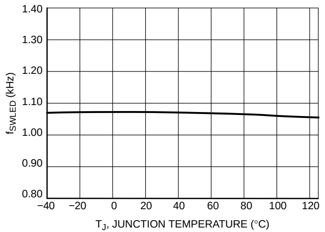
Figure 24. LED Switching Frequency at V CC = 15 V
