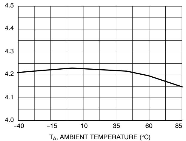
Figure 9. Soft-Start Current vs. Ambient Temperature
