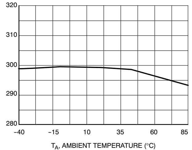
Figure 7. Switching Frequency vs. Ambient Temperature
