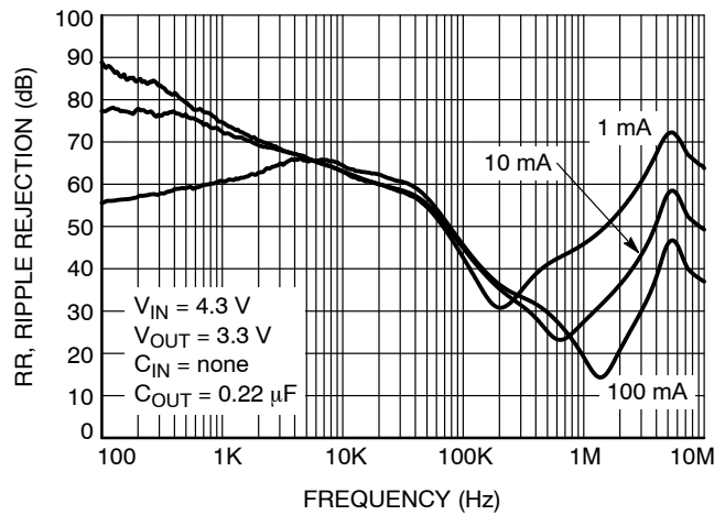
Figure 26. Power Supply Rejection Ratio, V_{OUT} = 3.3\text{ V} , C_{OUT} = 0.22\text{ }\mu\text{F}
