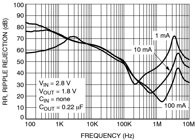
Figure 25. Power Supply Rejection Ratio, V_{OUT} = 1.8\text{ V} , C_{OUT} = 0.22\text{ }\mu\text{F}
