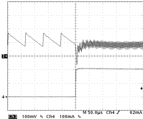
Upper Trace: Output Voltage Ripple, 100 mV/Division Lower Trace: Load Current, I_{LOAD} , 100 mA/Division ( V_{OUT} = 3.3\text{ V} , I_{LOAD} = 10\text{ mA to }200\text{ mA} ; L = 5.6\ \mu\text{H} , C_{OUT} = 22\ \mu\text{F} )
