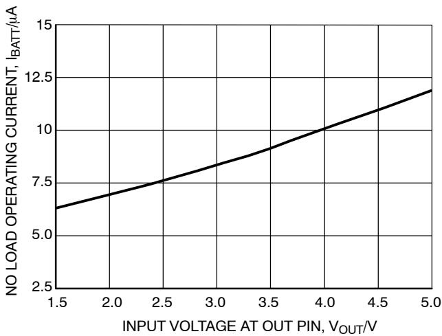
Figure 12. No Load Operating Current vs. Input Voltage at OUT Pin
