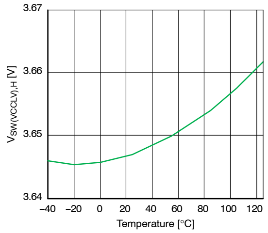
Figure 20. V SW(VCCCL),H vs. Temperature
