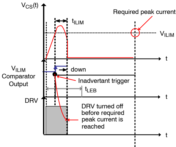
Figure 28. Circuit without Leading Edge Blanking
