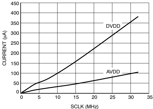
Figure 9. Current vs. SCLK Frequency
