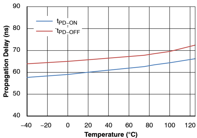
Figure 16. Propagation Delay
