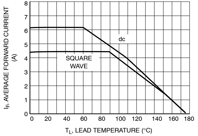
Figure 3. Current Derating Lead
