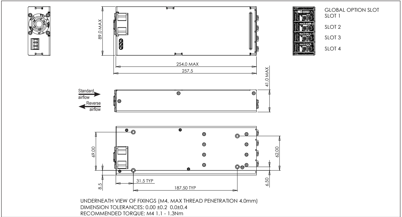
Units with factory fitted fan ('F' or 'R' type cooling)
