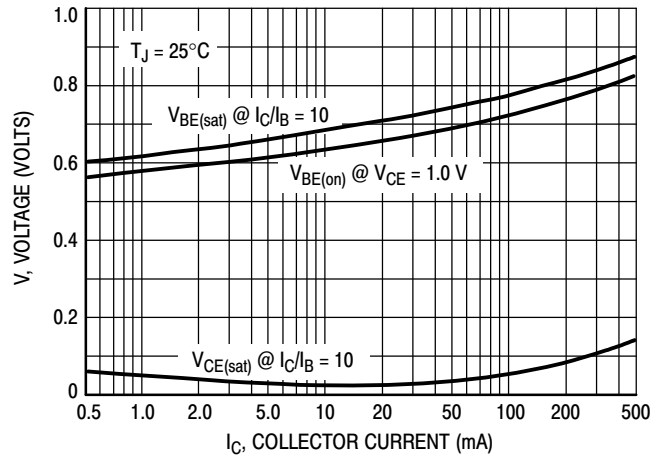
Figure 3. "On" Voltages
