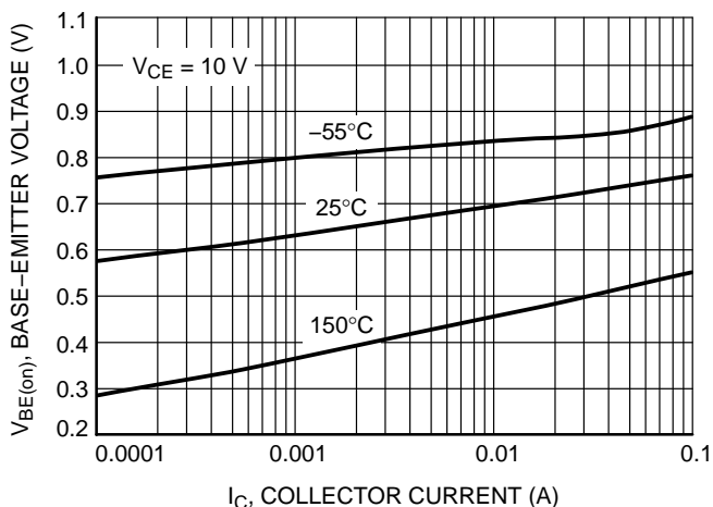
Figure 6. Base-Emitter Voltage vs. Collector Current
