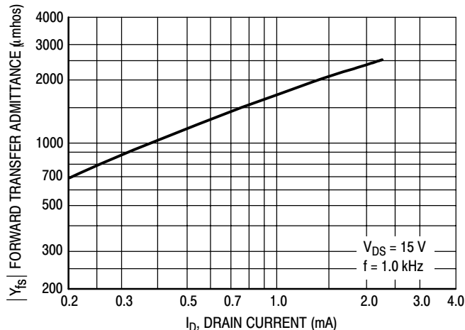
Figure 4. V_{GS(off)} = 2.0 Volts
