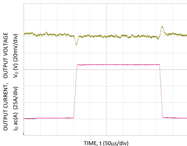
Figure 4. Trans. Resp. to 10A/μs Load Change from 25% to 75% at 12V IN , C_o=4 \times 0.047\mu\text{F} + 4 \times 0.1\mu\text{F} + 15 \times 22\mu\text{F} + 73 \times 47\mu\text{F} + 6 \times 470\mu\text{F} polymer.
