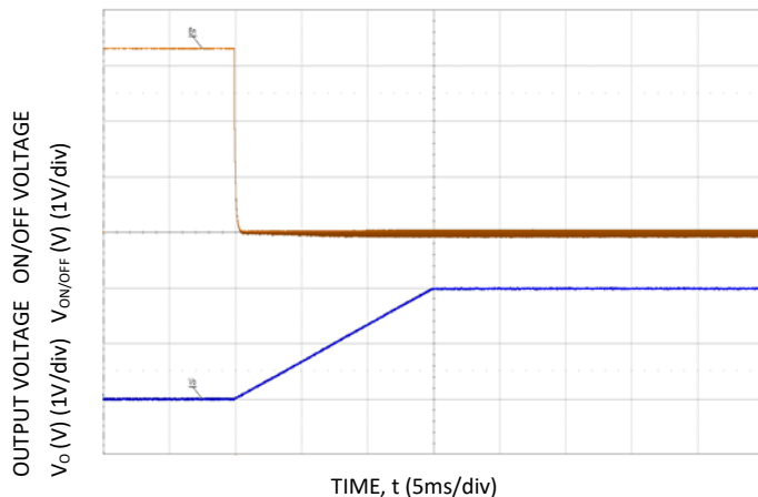
Figure 23. Typical Start-up Using On/Off Voltage ( I_o = I_{o\text{max}} ).
