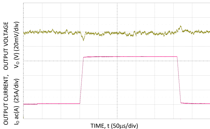
Figure 22. Trans. Resp. to 100A/μs Load Change from 25% to 75% at 12V_{IN} , C_o=4 \times 0.047\mu\text{F} + 4 \times 0.1\mu\text{F} + 15 \times 22\mu\text{F} + 73 \times 47\mu\text{F} + 6 \times 470\mu\text{F} polymer.
