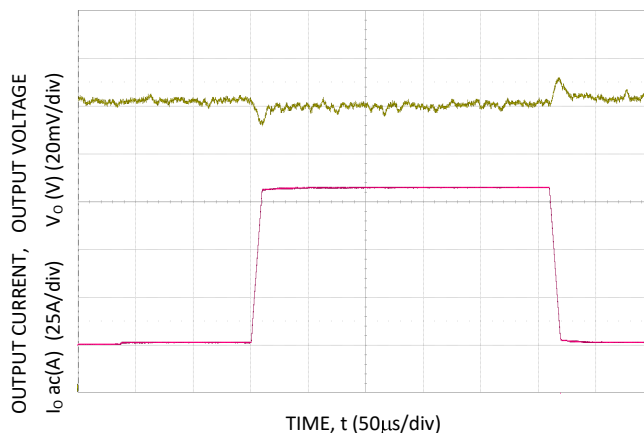
Figure 10. Trans. Resp. to 100\text{A}/\mu\text{s} Load Change from 25% to 75% at 12\text{V}_{IN} , C_o = 4 \times 0.047\mu\text{F} + 4 \times 0.1\mu\text{F} + 15 \times 22\mu\text{F} + 73 \times 47\mu\text{F} + 6 \times 470\mu\text{F} polymer.
