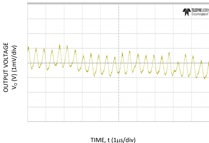
Figure 9. Typical output ripple ( C_o = 4 \times 0.047\mu\text{F} + 4 \times 0.1\mu\text{F} + 15 \times 22\mu\text{F} + 73 \times 47\mu\text{F} + 6 \times 470\mu\text{F} polymer, V_{IN} = 12\text{V} , I_o = I_{o,max} ).
