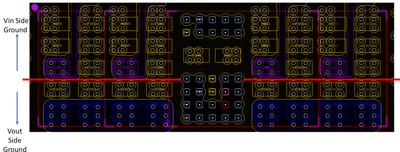
Figure 30. Example of split input-output ground
