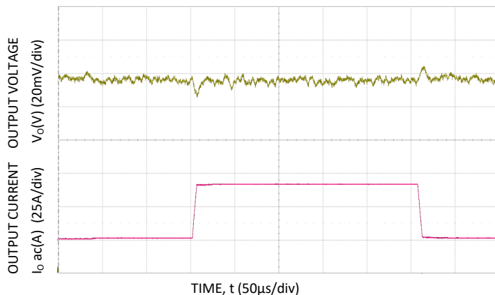
Figure 22. Trans. Resp. to 10\text{A}/\mu\text{s} Load Change from 25% to 75% at 12\text{V}_{IN} , C_o=4 \times 0.047\mu\text{F} + 4 \times 0.1\mu\text{F} + 15 \times 22\mu\text{F} + 73 \times 47\mu\text{F} + 6 \times 470\mu\text{F} polymer
