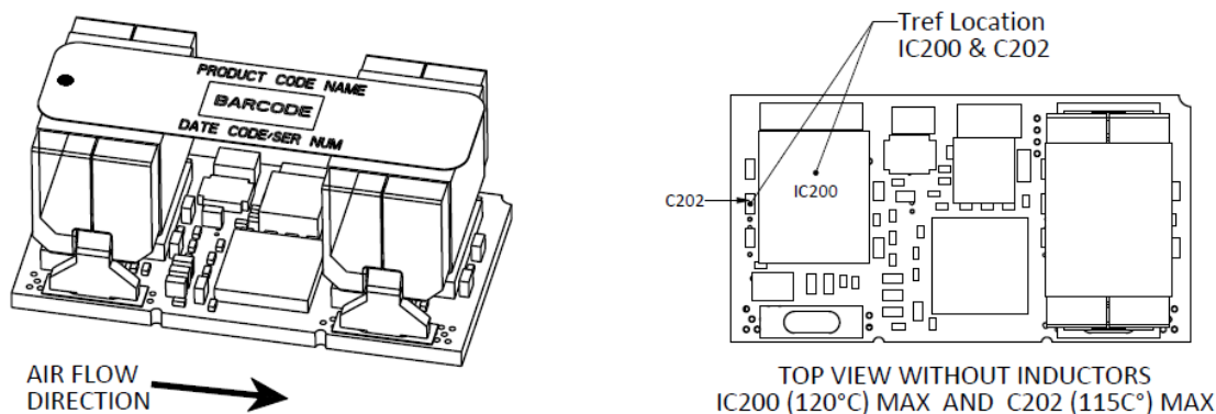
Figure 29. Preferred airflow direction and the location of the thermal reference points
