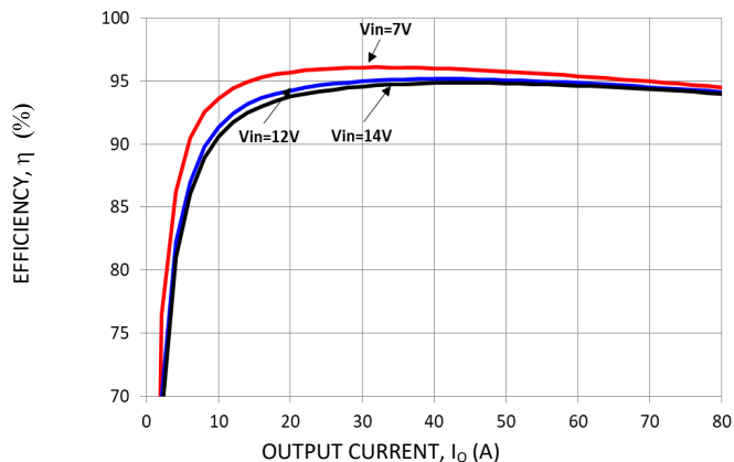
Figure 19. Converter Efficiency versus Output Current.
