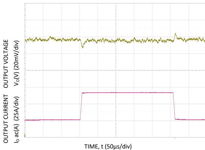
Figure 16. Trans. Resp. to 10A/μs Load Change from 25% to 75% at 12\text{V}_{IN} , C_o=4 \times 0.047\mu\text{F} + 4 \times 0.1\mu\text{F} + 15 \times 22\mu\text{F} + 73 \times 47\mu\text{F} + 6 \times 470\mu\text{F} polymer
