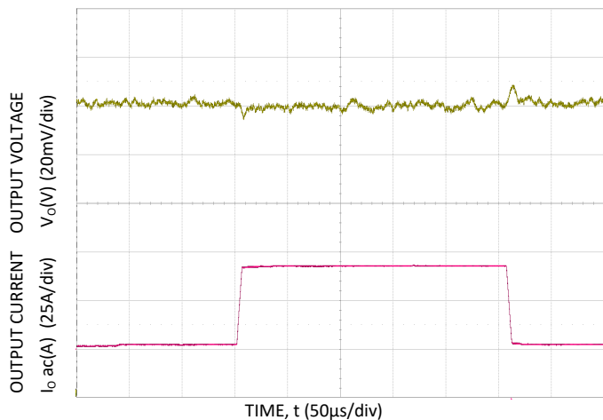
Figure 10. Trans. Res. to 10\text{A}/\mu\text{s} Load Change from 25% to 75% at 12\text{V}_{IN} , C_o=4 \times 0.047\mu\text{F} + 4 \times 0.1\mu\text{F} + 15 \times 22\mu\text{F} + 73 \times 47\mu\text{F} + 6 \times 470\mu\text{F} polymer
