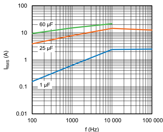
Maximum RMS current as function of frequency T_{amb} \leq 85^\circ C ; U_r = 250 V_{AC}
