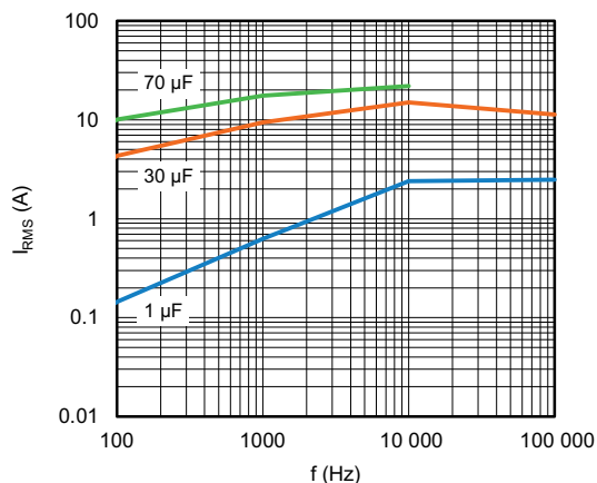
Maximum RMS current as function of frequency T_{amb} \leq 85^\circ C ; U_r = 230 V_{AC}
