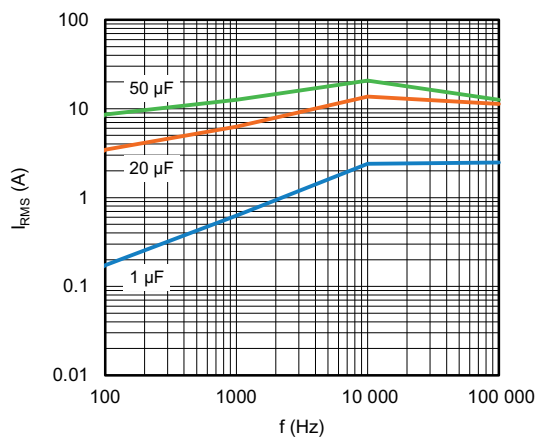
Maximum RMS current as function of frequency T_{amb} \leq 85^\circ C ; U_r = 275 V_{AC}
