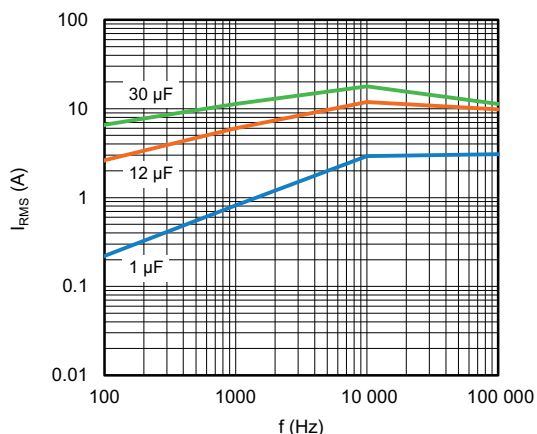
Maximum RMS current as function of frequency T_{amb} \leq 85^\circ C ; U_r = 350 V_{AC}
