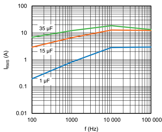
Maximum RMS current as function of frequency T_{amb} \leq 85^\circ C ; U_r = 310 V_{AC}
