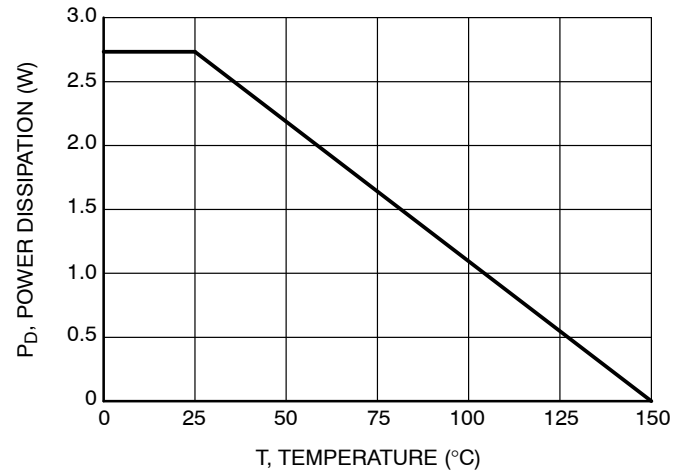
Figure 8. Power Derating
