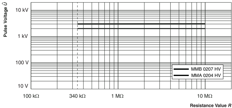
Pulse load rating in accordance with IEC 60115-1, 4.27; 10 μs/700 μs; 10 pulses at 1 minute intervals; for permissible resistance change (0.5 % R + 0.05 Ω)
