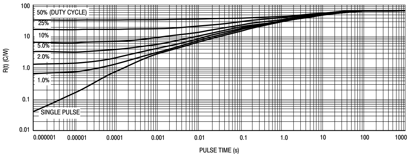
Figure 9. Thermal Response, Junction-to-Ambient (1 in 2 pad)
