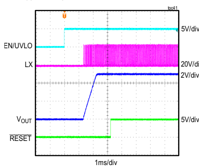
MAXM17634 STARTUP THROUGH ENABLE V_{OUT} = 5V , f_{SW} = 1MHz , FULL LOAD, PWM MODE
