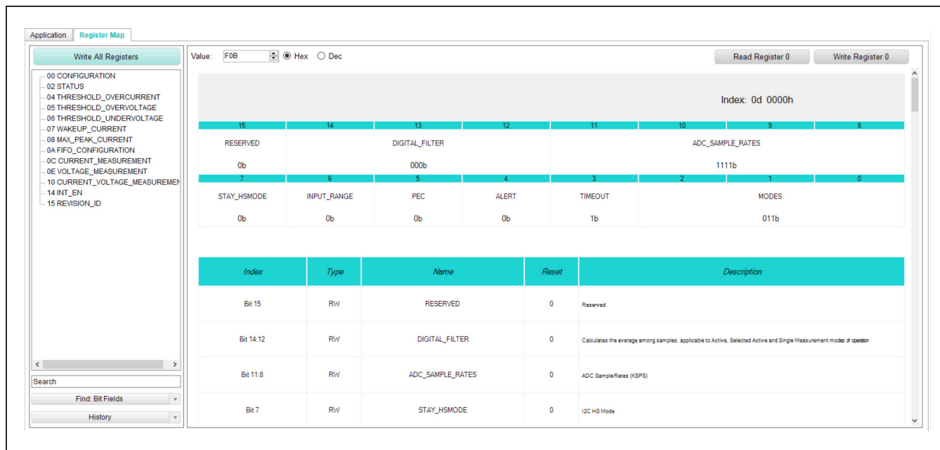
Figure 3. Register Map
