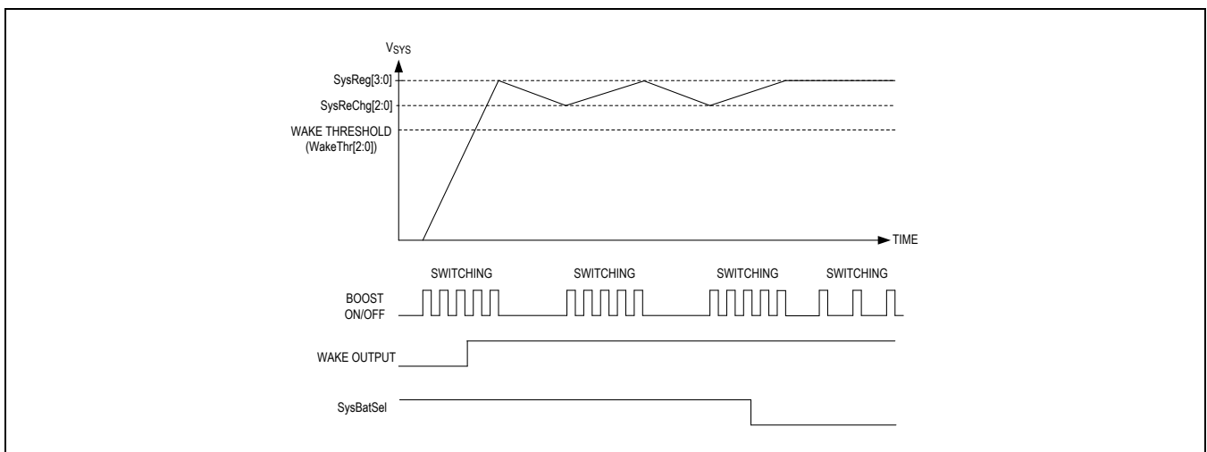
Figure 2. Waveform of VSYS and WAKE Output
