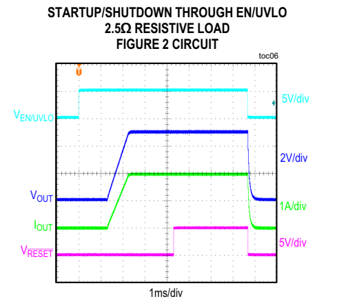
CONDITION: \overline{\text{RESET}} IS PULLED UP TO V CC WITH A 10kΩ RESISTOR
