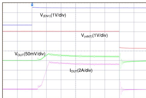
Time (200 \mu\text{s}/\text{div} )
