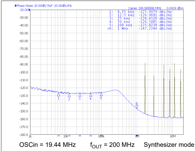
Figure 6-2. Typical Closed-Loop Phase Noise
