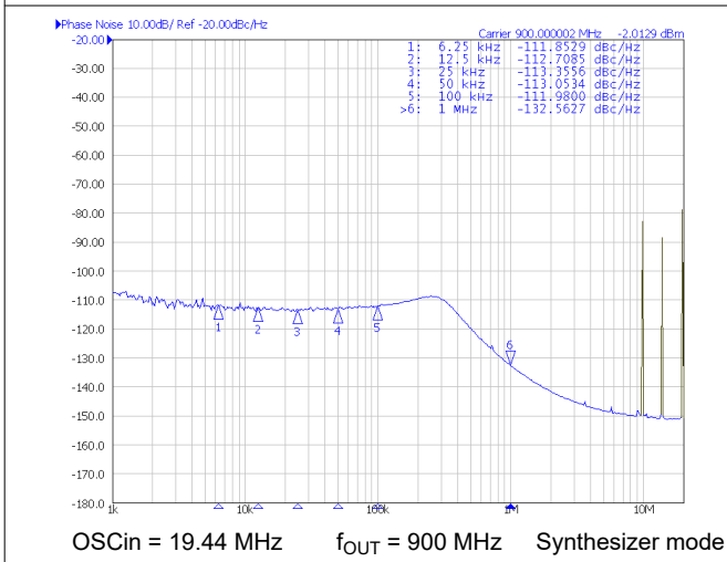
Figure 6-4. Typical Closed-Loop Phase Noise
