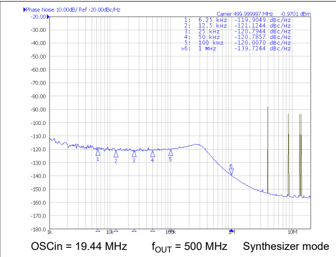
Figure 6-3. Typical Closed-Loop Phase Noise
