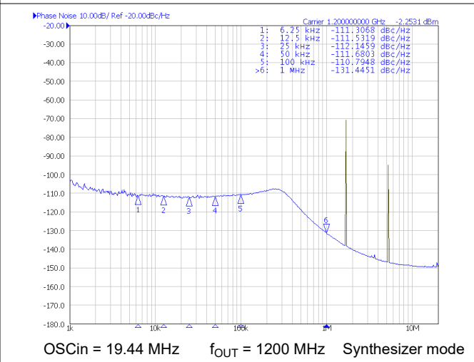
Figure 6-5. Typical Closed-Loop Phase Noise
