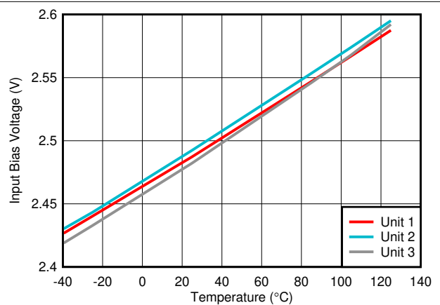
Gain = 20 kΩ
