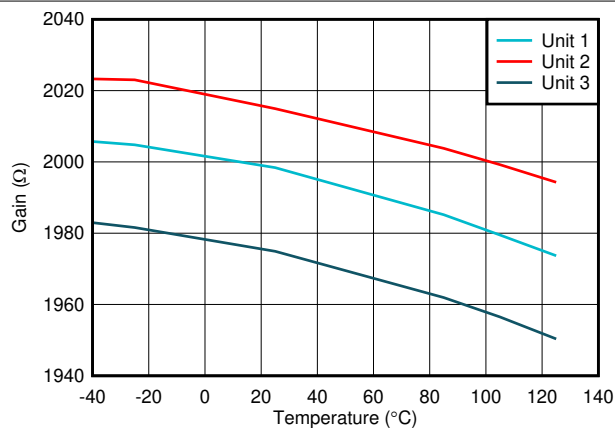
Gain = 2 kΩ
