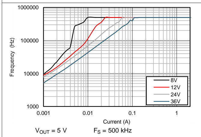
Figure 59. Frequency vs Load
