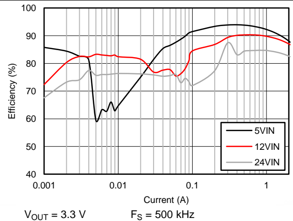
Figure 42. Efficiency at 85°C
