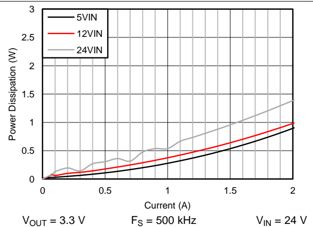
Figure 44. Power Loss at 85°C
