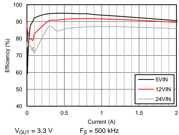
Figure 40. Efficiency at Room Temperature
