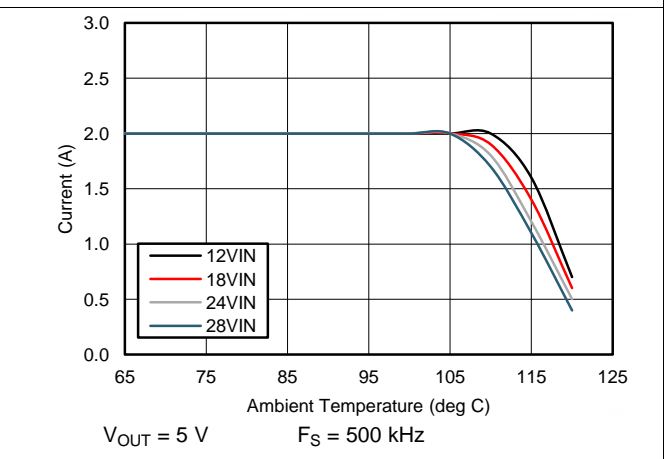
Figure 62. Derating Curve
