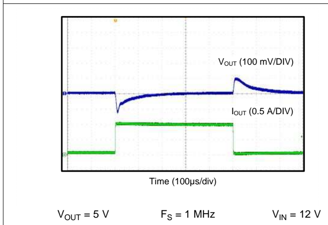
Figure 61. Load Transient 0.1 A to 1 A
