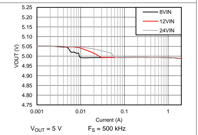
Figure 60. Regulation Curve
