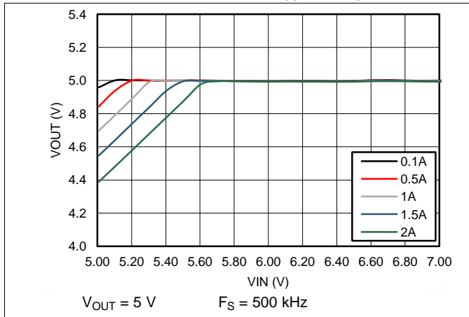
Figure 57. Dropout Voltage
