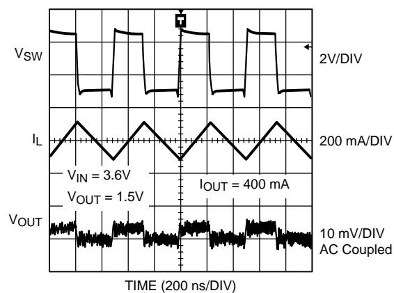
Figure 18. PWM Operation
