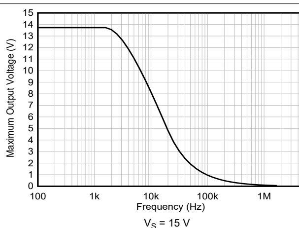
Figure 6-32. Maximum Output Voltage vs Frequency V_S = 15\text{ V}
