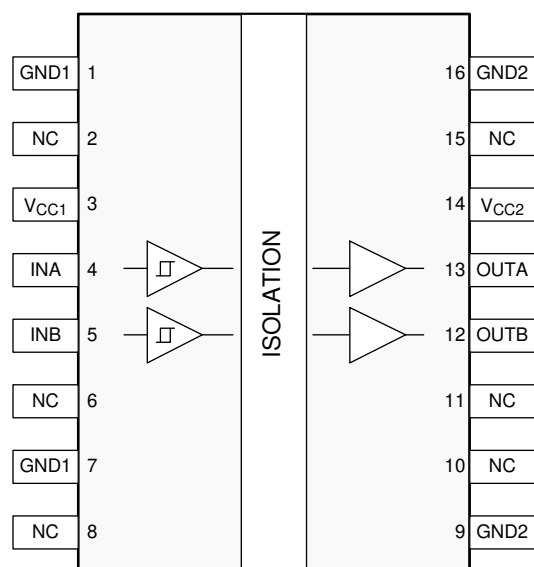
Figure 5-1. ISO7720 DW Package 16-Pin SOIC Top View
