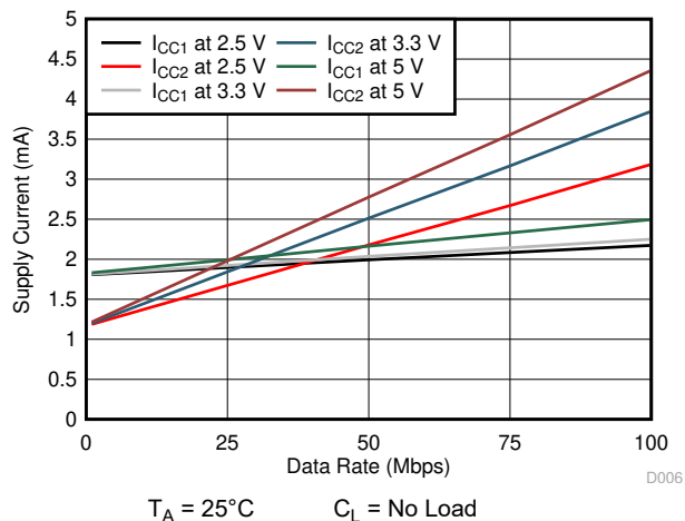
Figure 6-8. ISO7720 Supply Current vs Data Rate (With No Load)
