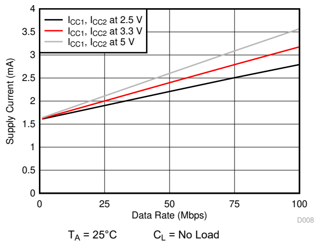
Figure 6-10. ISO7721 Supply Current vs Data Rate (With No Load)
