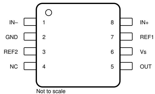
Figure 6-2. INA241x-Q1: D and DGK Package 8-Pin SOIC and 8-Pin VSSOP Top View 1. D (SOIC) package is preview only.
