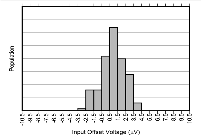
Figure 7-2. INA241A2-Q1 Input Offset Production Distribution
