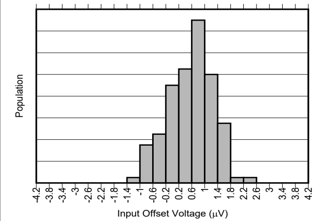
Figure 7-4. INA241A5-Q1 Input Offset Production Distribution
