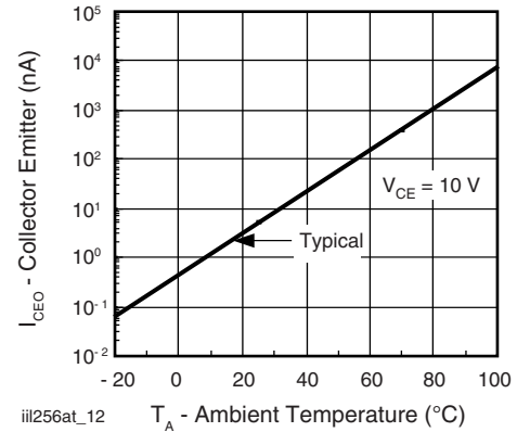
Fig. 12 - Collector-Emitter Leakage Current vs.Temp.
