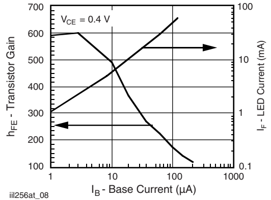
Fig. 8 - Base Current vs. I_F and h_{FE}
