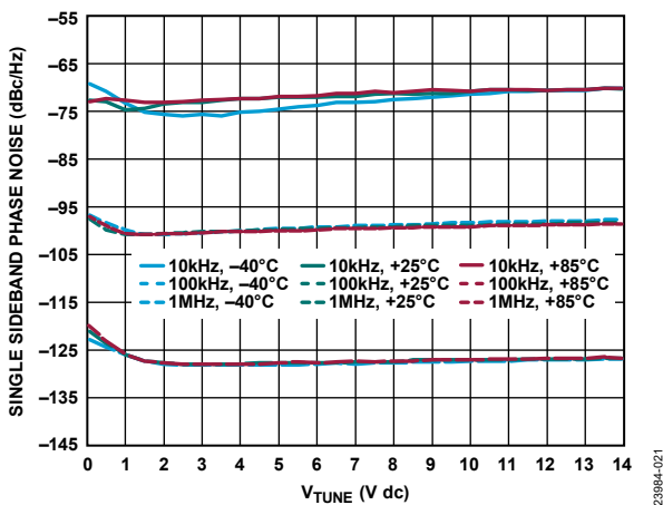
Figure 19. Single Sideband Phase Noise vs. V_{TUNE} for Various Temperatures and Frequencies
