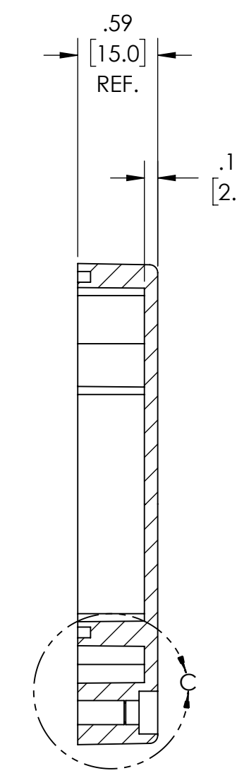
SECTION B-B
