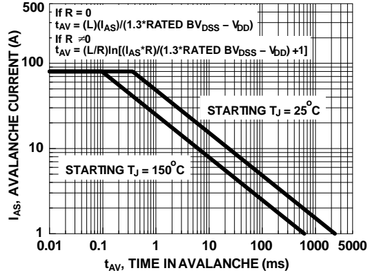
NOTE: Refer to Application Notes AN7514 and AN7515 Figure 4. Unclamped Inductive Switching Capability
