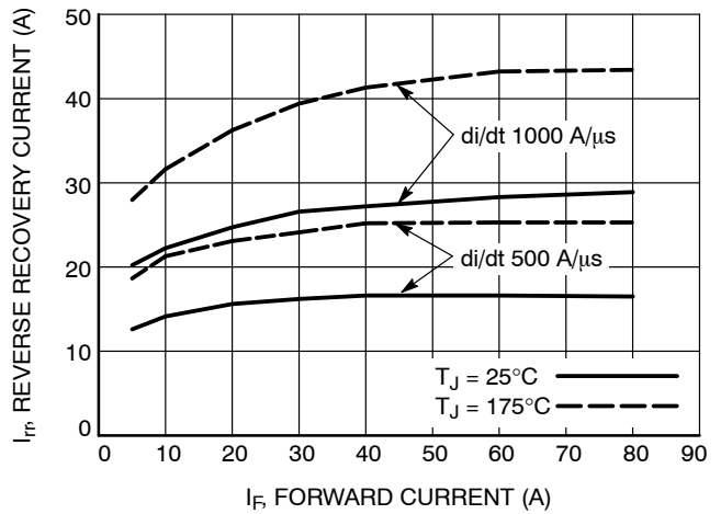
Figure 16. (Diode) Reverse Recover Current vs. Forward Current
