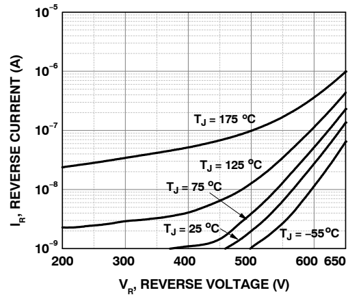
Figure 2. Reverse Characteristics
