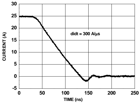
Figure 27. FDMS3664S SyncFET™ body diode reverse recovery characteristic
