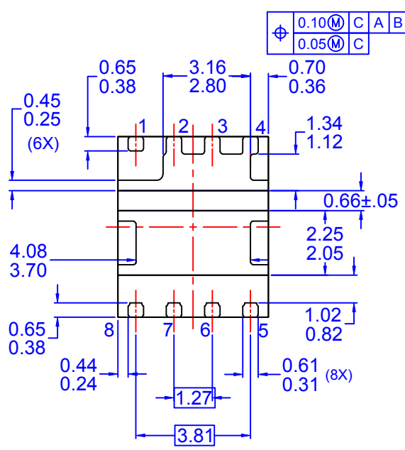
BOTTOM VIEW OPTION - A (SAWN TYPE)
