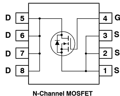
N-Channel MOSFET
