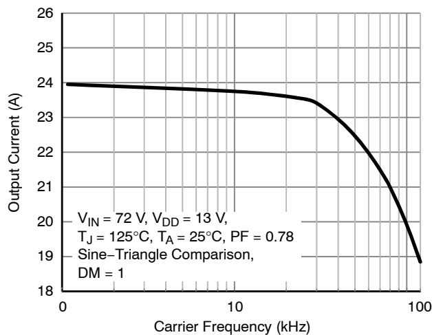
Figure 37. Output Current vs. Carrier or Modulation Frequency
