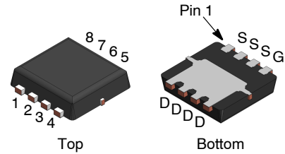
WDFN8 3.3x3.3, 0.65P CASE 511DR
